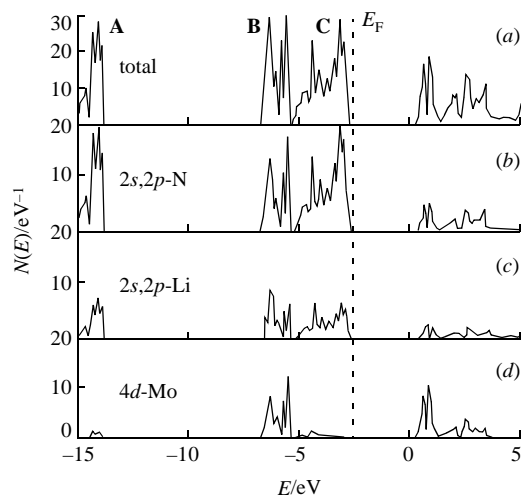
Figure 1 The (a) total and (b)–(d) partial densities of states [N(E)] for a \text{Li}_6\text{MoN}_4 crystal.
