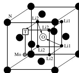
Figure 2 The structure of a perfect crystal of \text{Li}_6\text{MoN}_4 . Arrows show possible transitions for lithium ions into octahedral interstitial position (O) and through structure tetravacancies (T).
